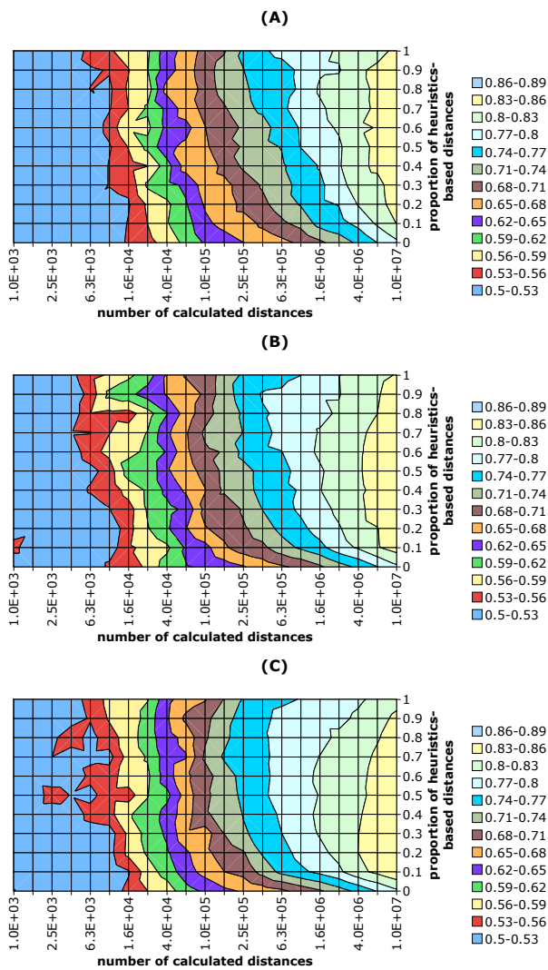
Supplementary Fig. 1: HappieClust JDR quality for data=Shyamsundar05 and different numbers of pivots: (A) q = 5 ; (B) q = 10 ; (C) q = 20 .
